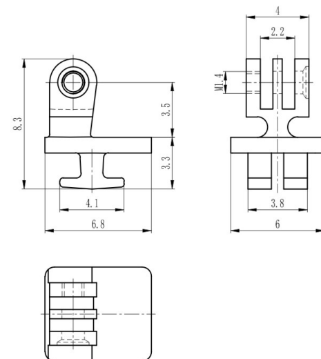
塑铰 Regular hinge for plastic frame XAA4060-60-WN 材料/Material: 无铅白铜/Lead free nickel silver
