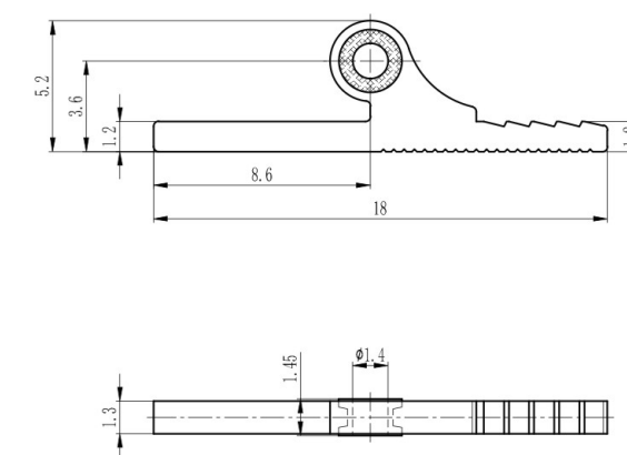
加胶注塑铰链 Safely injection hinge XAD4001A14-WN
