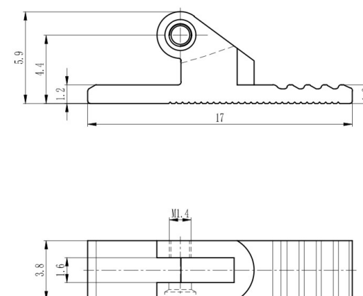
注塑铰链 Injection hinge XAC4224A38-WN
