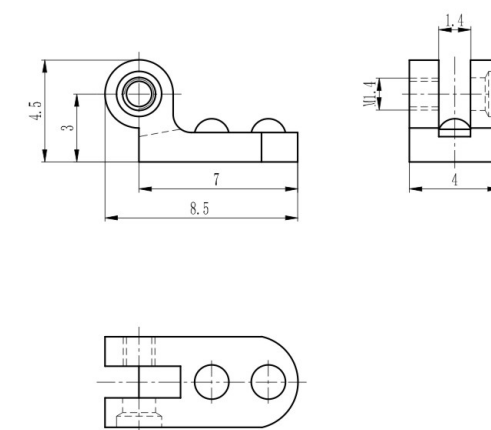
塑铰 Regular hinge for plastic frame XAE4178-40-WV 材料/Material: 无铅白铜/Lead free nickel silver
