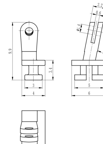
塑铰 Regular hinge for plastic frame XAA4047A60-WN
